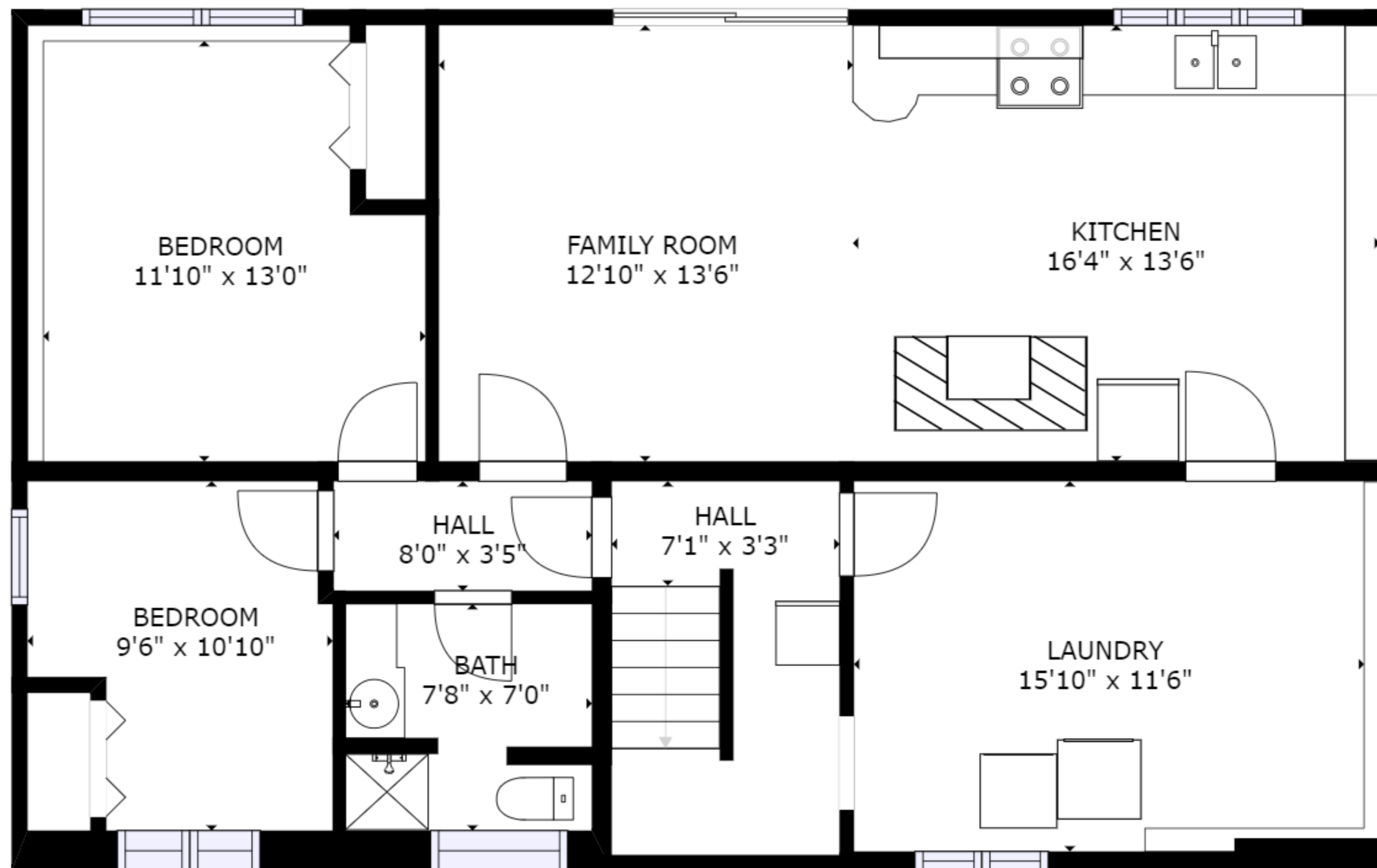
FLOOR 2
