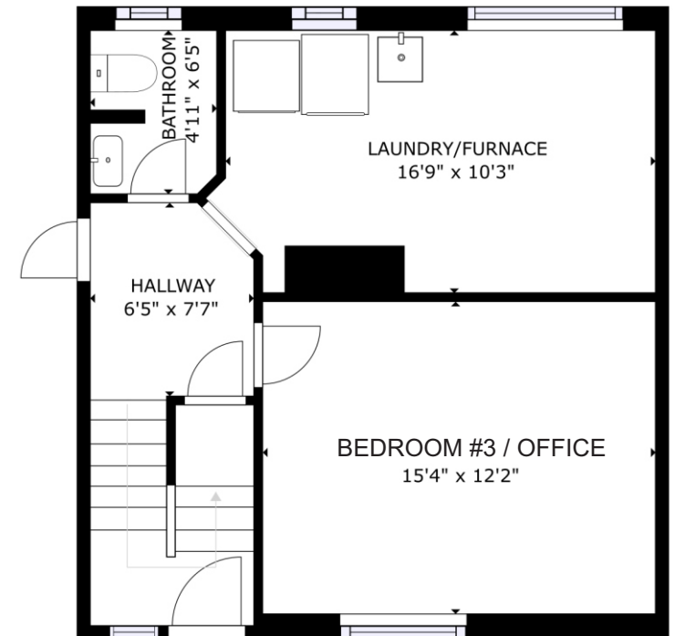
LOWER FLOOR
