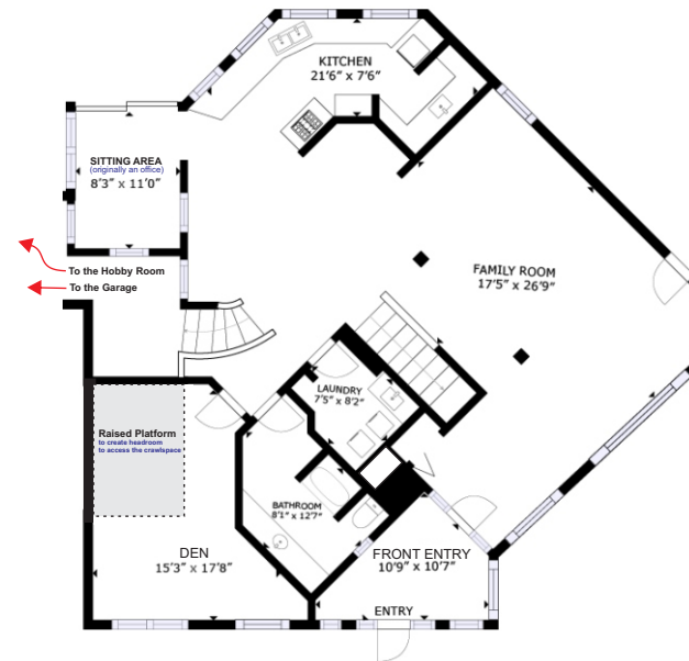
Main Floor
